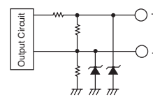
Output Circuit
