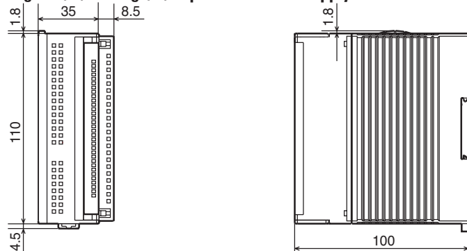
Digital I/O, Analog I/O, Expansion Power Supply
